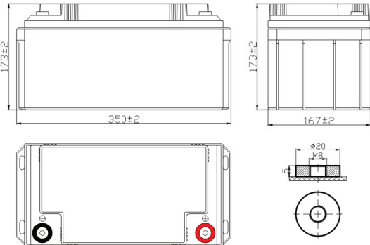
Unit:(mm) Terminal type:(T3)
